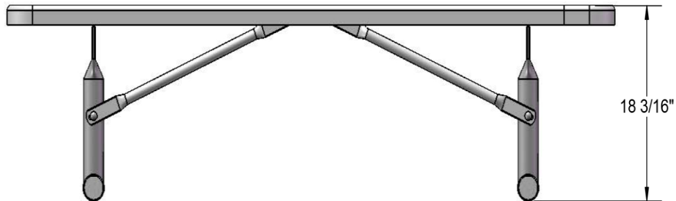
Front View:
