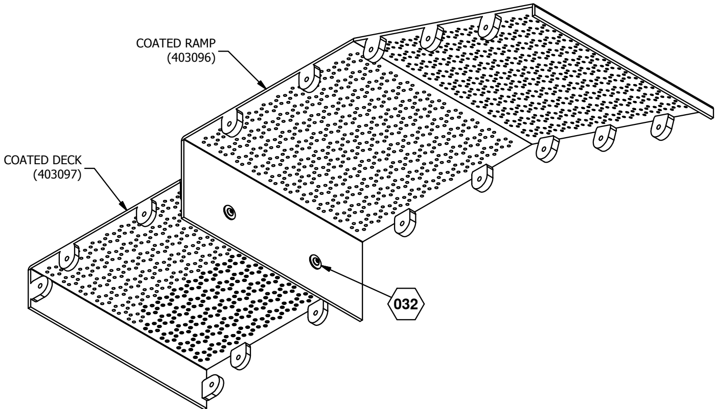
UNDERNEATH VIEW
