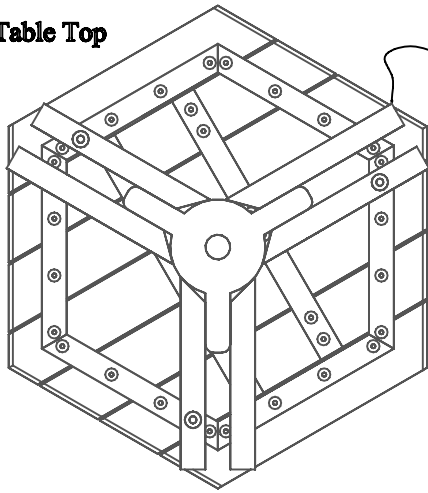
F - Small Spoke Assembly
