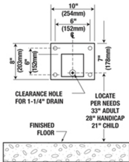
VIEW FOR MOUNTING
