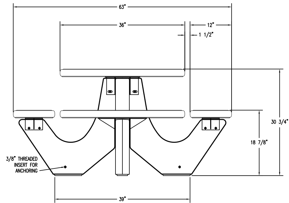
2 ELEVATION VIEW
