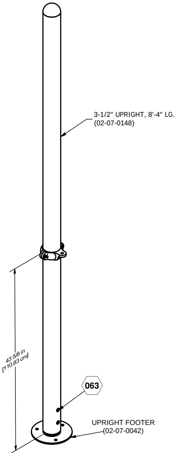
FINISHED ASSEMBLY
