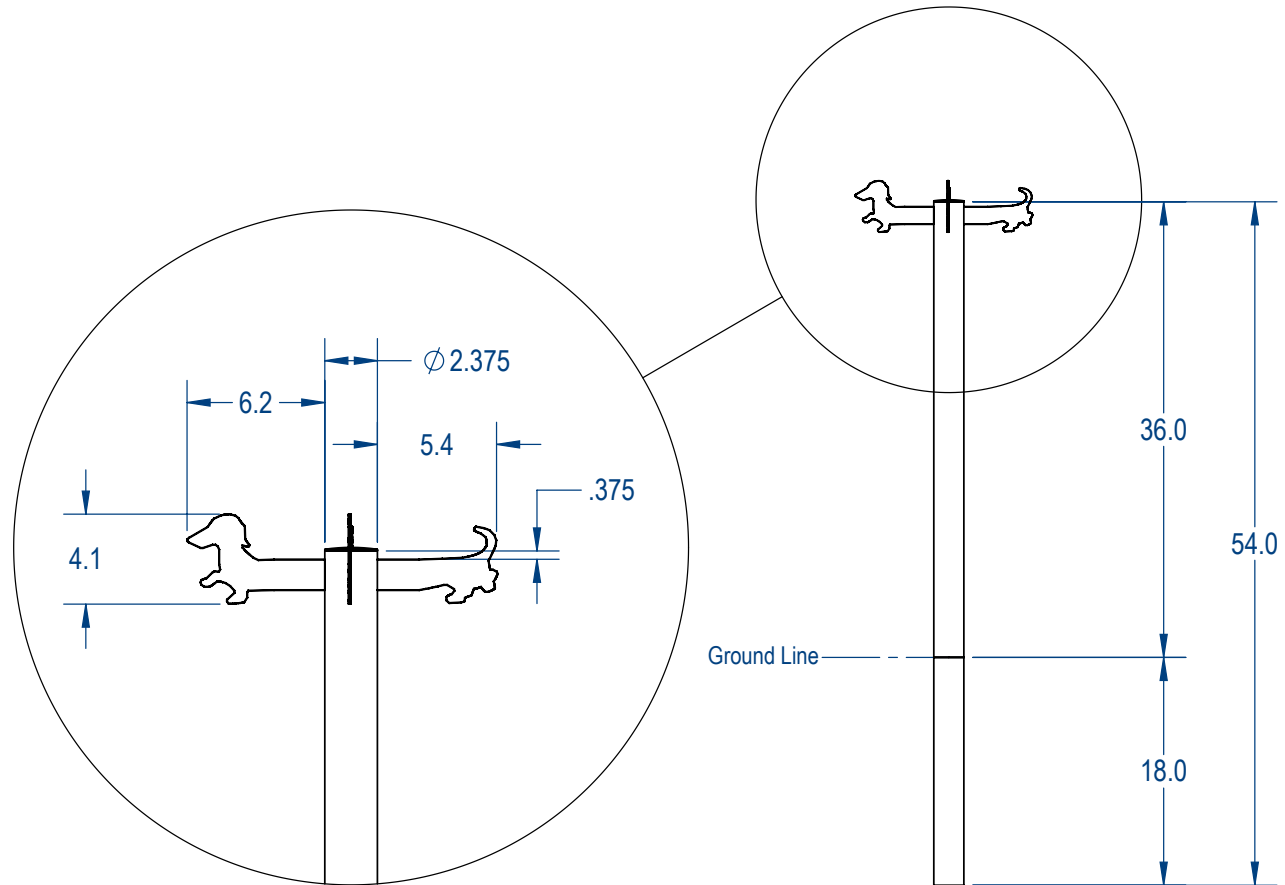
DETAIL A SCALE 1 : 8
