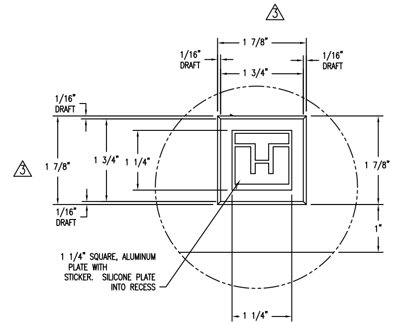
5 DETAIL FOR EMBLEM RECESS Scale: 1" = 1"
