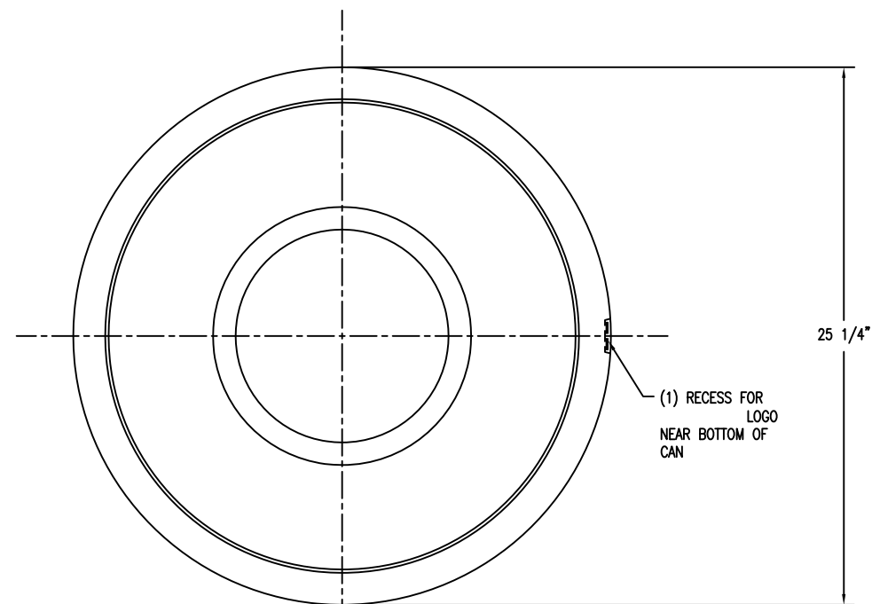
3 TOP VIEW Scale: 1/4" = 1"
