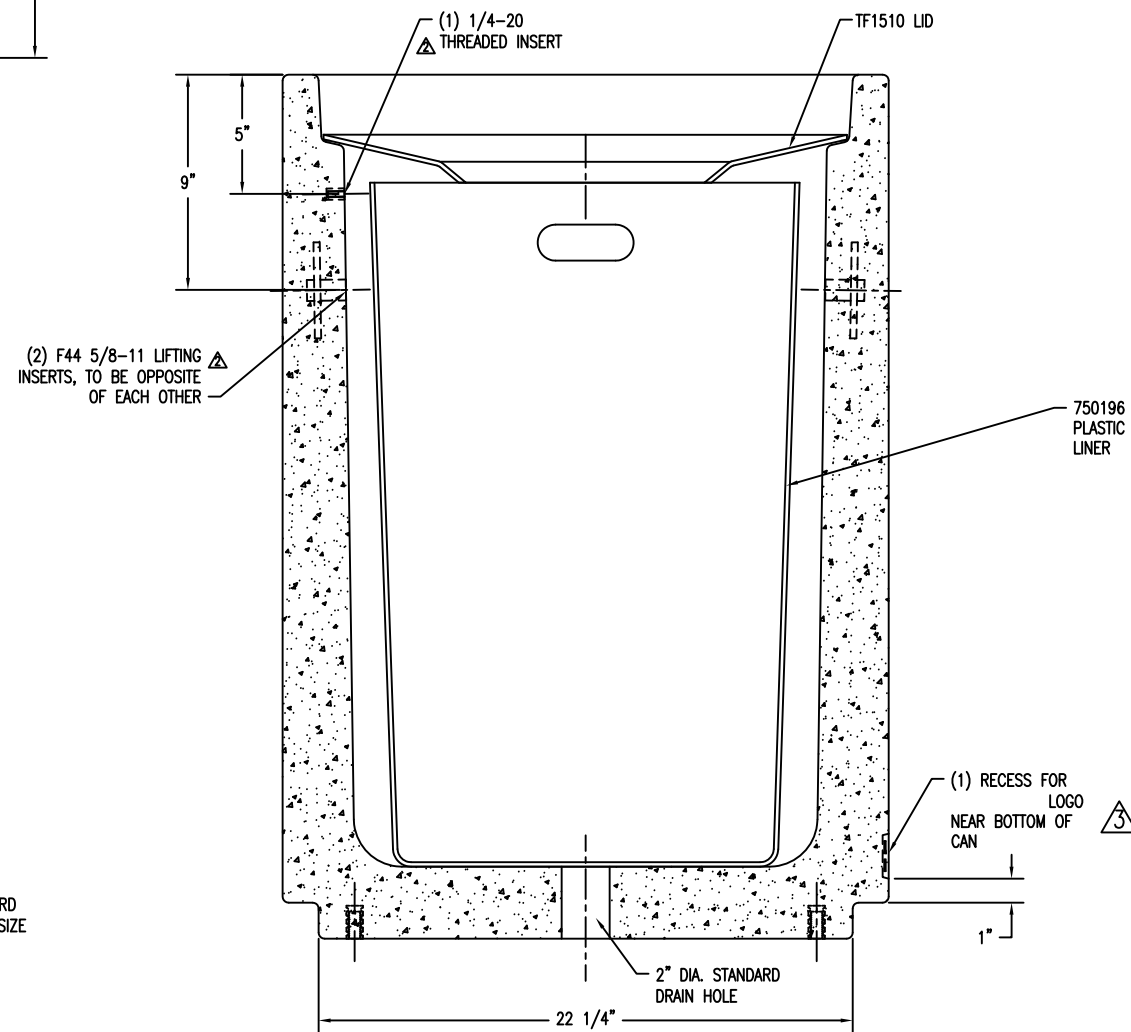
4 SECTION VIEW Scale: 1/4" = 1"
