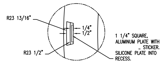
6 TOP VIEW OF RECESS BLOCK OUT FOR EMBLEM Scale: 1/2" = 1"
