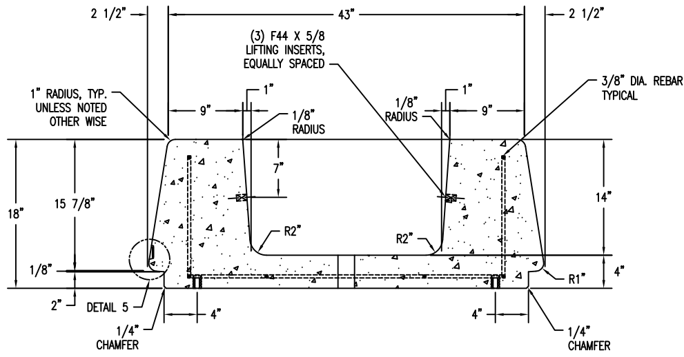
1 PLANTER CROSS SECTION Scale: 1/8" = 1"
