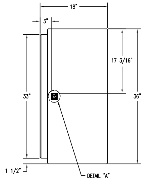
4 LEFT SIDE VIEW OF BENCH WS-119 Scale: 1/8" = 1"
