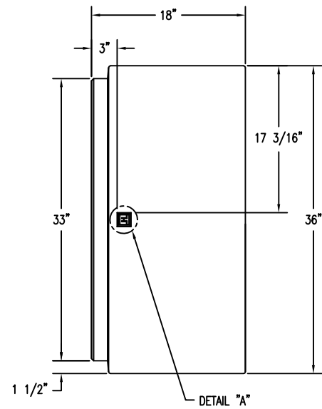
4 LEFT SIDE VIEW OF BENCH WS-118 Scale: 1/8" = 1"
