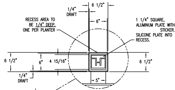
3 RECESS BLOCK OUT FOR EMBLEM Scale: 1/2" = 1"
