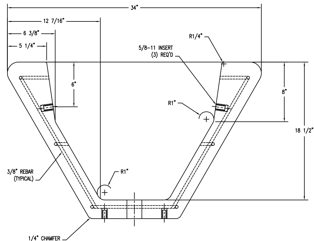
3 SECTION VIEW OF BENCH WS-106 Scale: 1/8" = 1"
