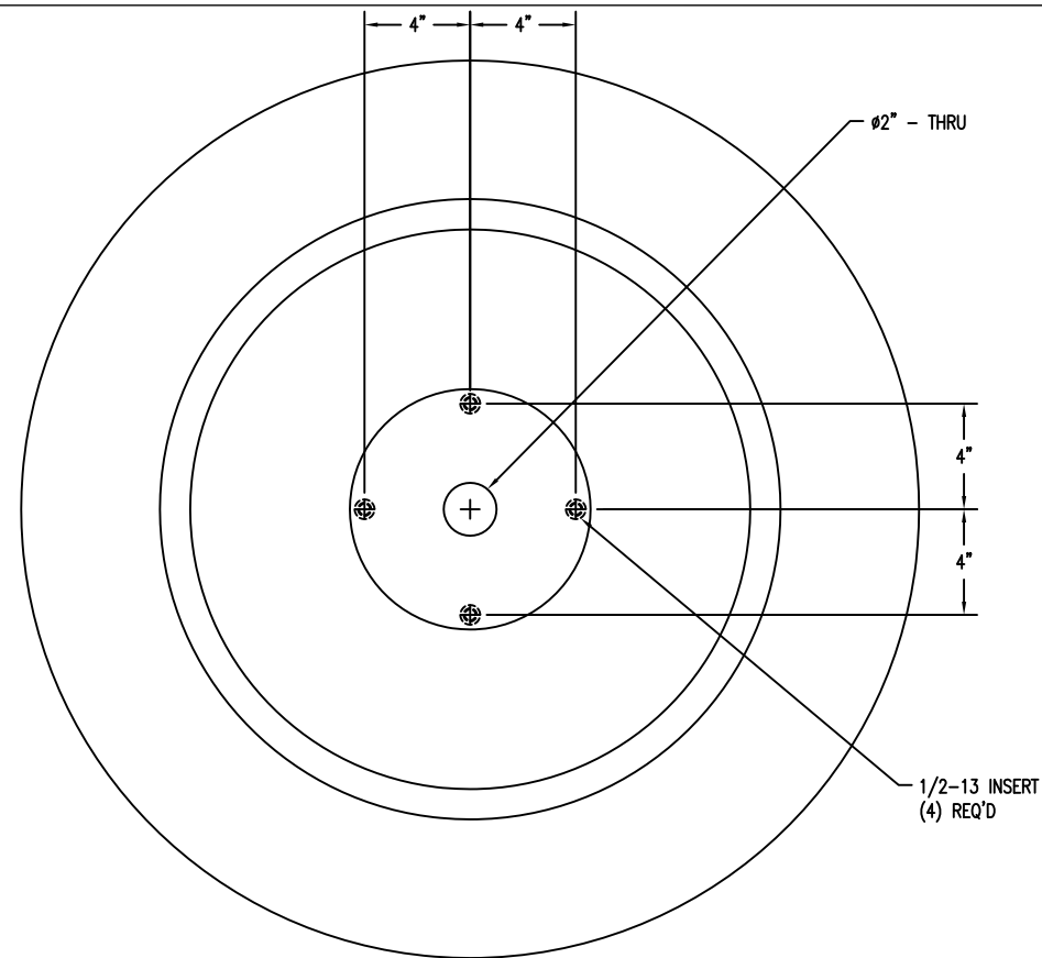
1 TOP VIEW OF BENCH WS-106 Scale: 1/8" = 1"
