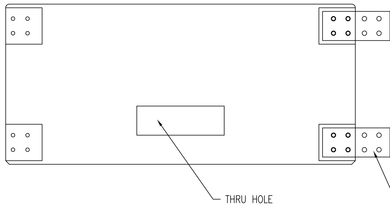
3 BACK ELEVATION OF DF5520 EXTENSION PANEL Scale: 1/8" = 1"
