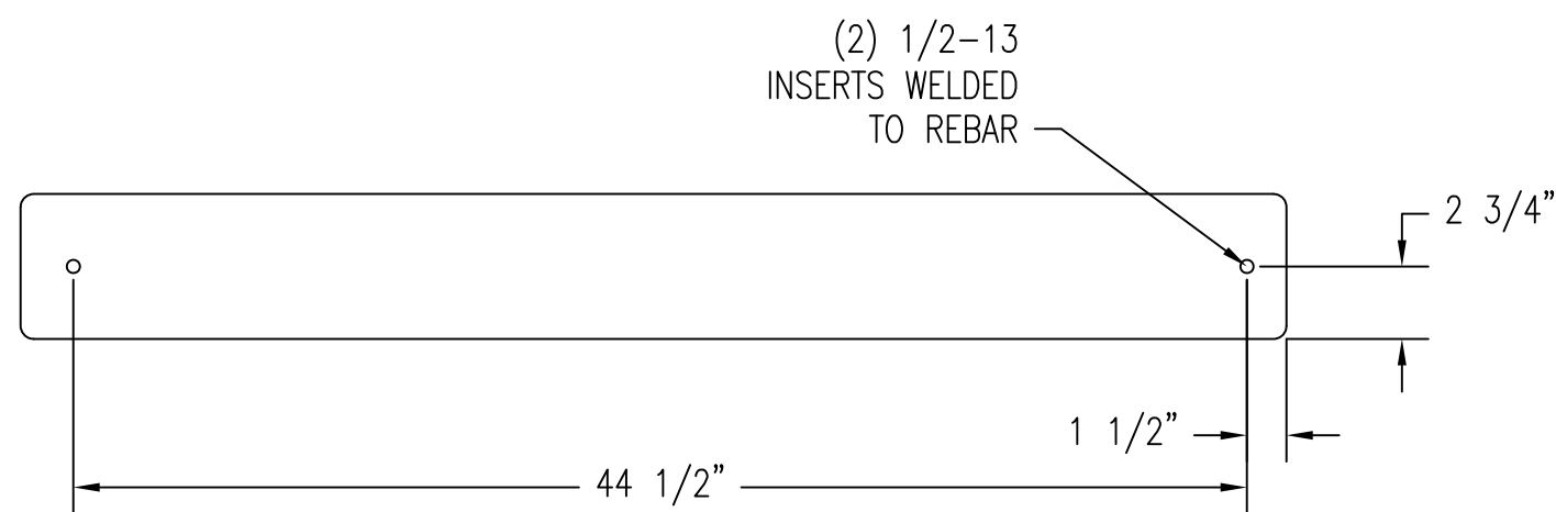
4 BOTTOM VIEW OF DF5520 EXTENSION PANEL Scale: 1/8" = 1"
