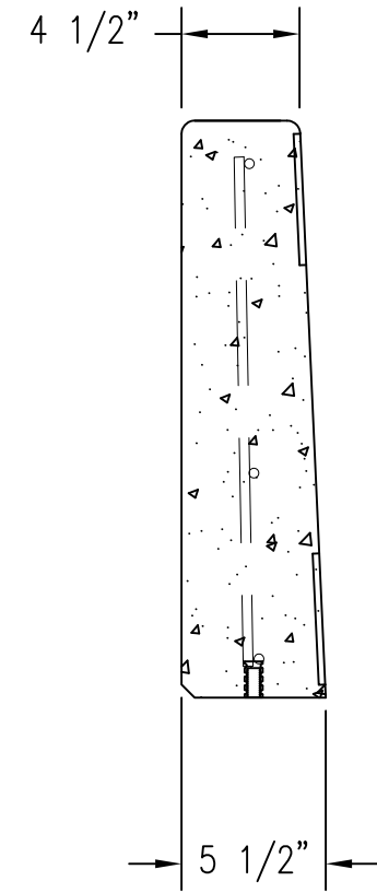
5 SECTION VIEW OF DF5520 EXTENSION PANEL Scale: 1/8" = 1"
