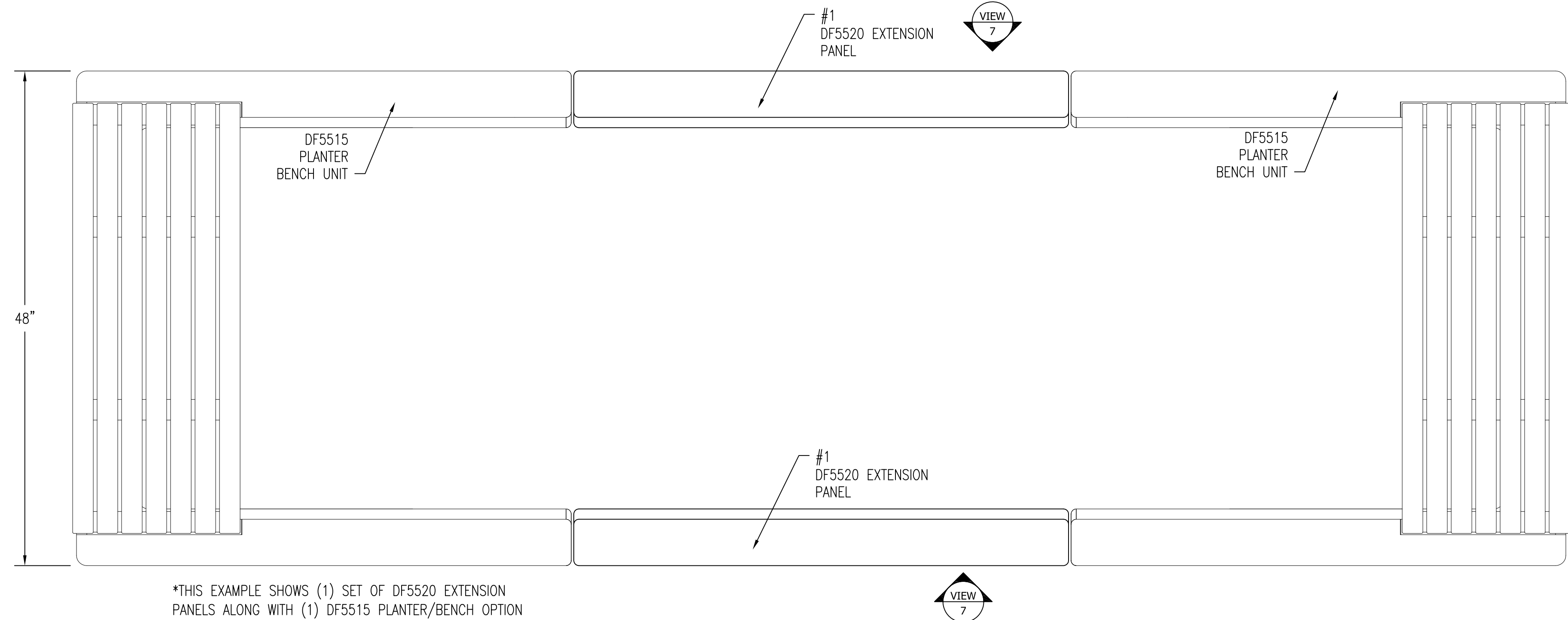
6 TOP VIEW OF DF5520 EXTENSION PANEL WITH DF5515 STANDARD PLANTER Scale: 1/8" = 1"
