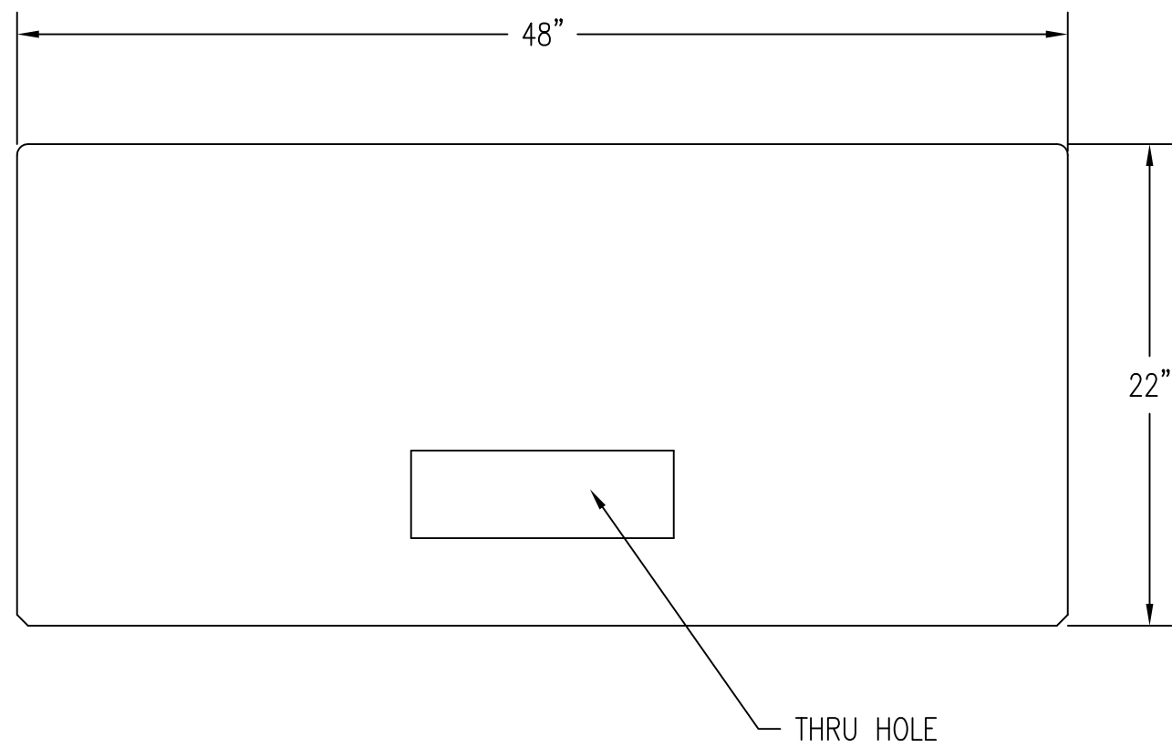
2 FRONT ELEVATION OF DF5520 EXTENSION PANEL Scale: 1/8" = 1"
