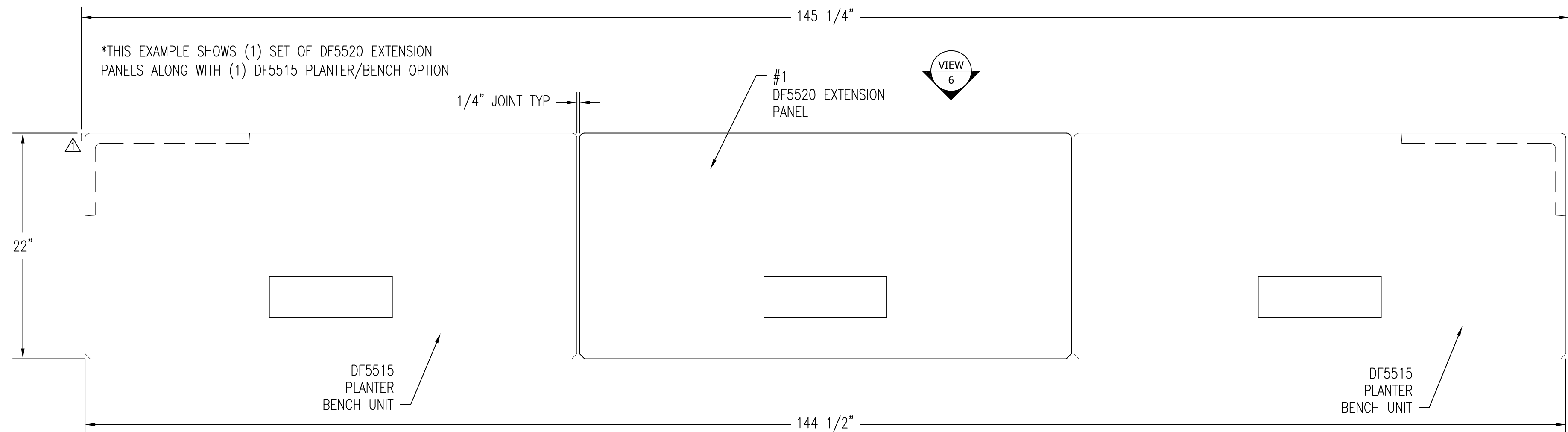
7 FRONT ELEVATION OF DF5520 EXTENSION PANEL WITH DF5515 STANDARD PLANTER Scale: 1/8" = 1"
