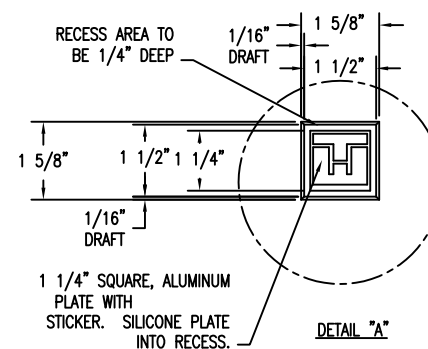
5 ENLARGE DETAIL OF LOGO & RECESS Scale: 1/2" = 1"
