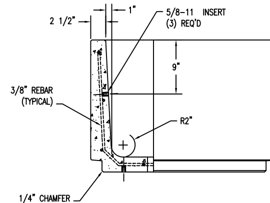
4 CROSS SECTION OF BENCH WS-117 Scale: 1/8" = 1"
