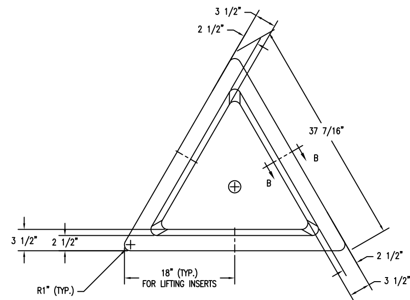
1 TOP VIEW OF BENCH WS-117 Scale: 1/8" = 1"
