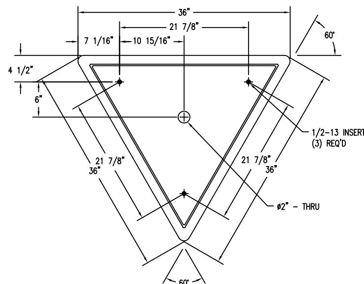
3 BOTTOM VIEW OF BENCH WS-117 Scale: 1/8" = 1"
