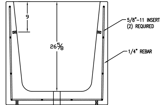
SECTION VIEW
