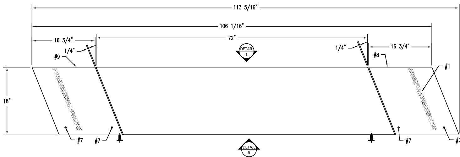
3 FRONT ELEVATION OF ASSEMBLED BENCH UNIT Scale: 1/8" = 1"
