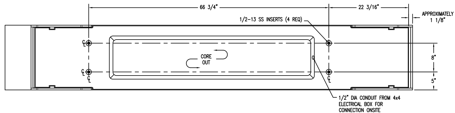
5 BOTTOM VIEW OF ASSEMBLED BENCH UNIT Scale: 1/8" = 1"
