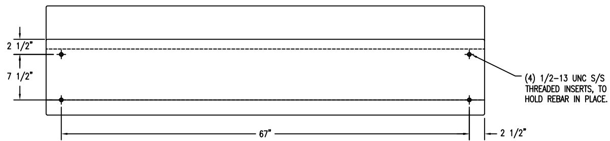
4 BOTTOM VIEW Scale: 1/4" = 1"
