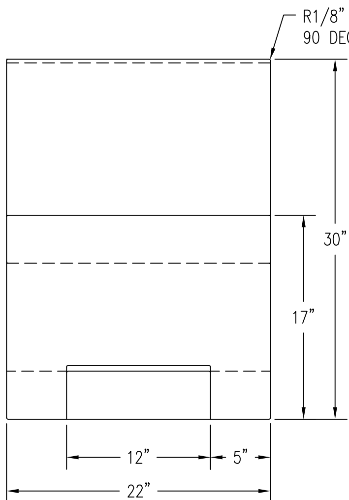
2 FRONT VIEW Scale: 1/8" = 1"
