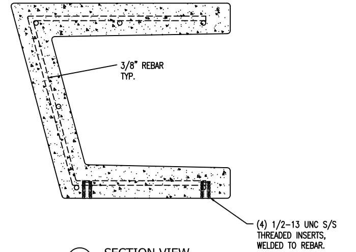
7 SECTION VIEW Scale: 1/4" = 1"
