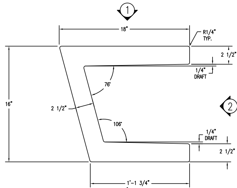
4 END VIEW Scale: 1/4" = 1"
