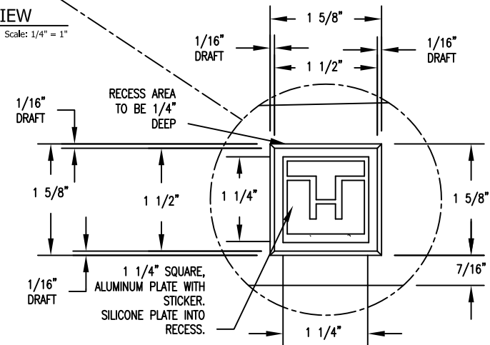
6 RECESS BLOCK OUT FOR EMBLEM Scale: 1" = 1"
