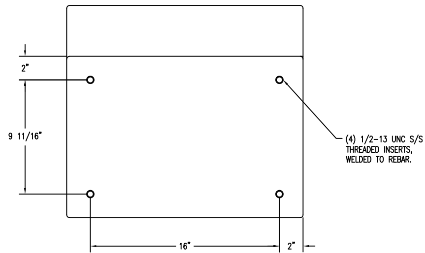
3 BOTTOM VIEW Scale: 1/4" = 1"
