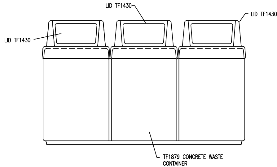
2 FRONT ELEVATION Scale: 1/16" = " 1"
