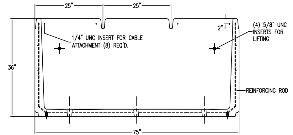
7 SECTION VIEW Scale: 1/16" = " 1"
