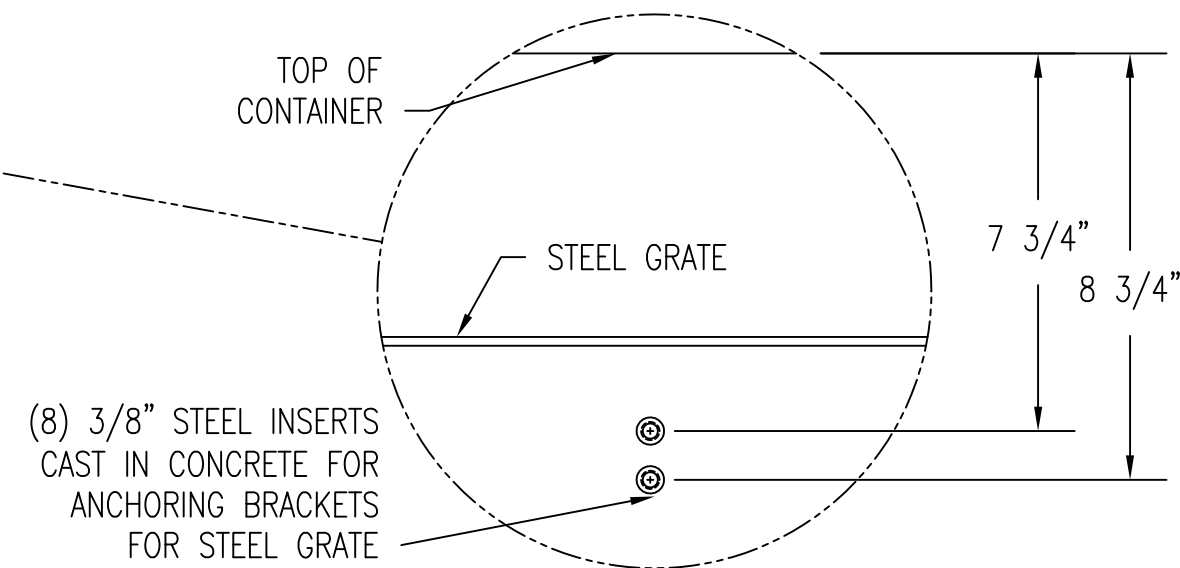
5 ENLARGED DETAIL FOR INSERTS Scale: 1/4" = 1"
