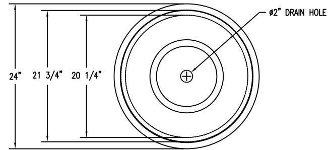
1 TOP VIEW OF TF1840 WASTE CONTAINER SHOWN WITHOUT LID Scale: 1/8" = 1"
