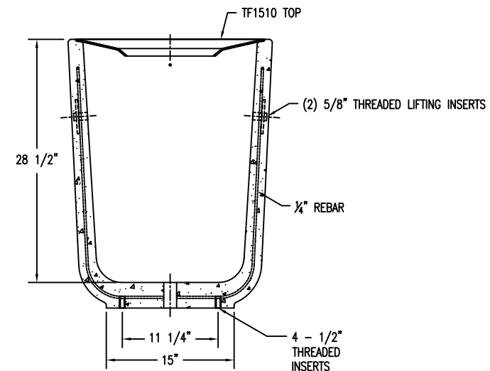
4 SECTION VIEW OF WASTE CONTAINER SHOWN WITHOUT LID Scale: 1/8" = 1"
