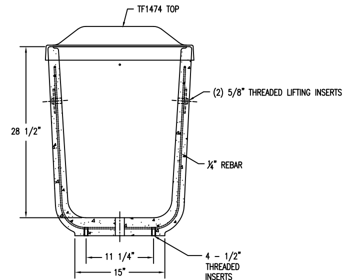
4 SECTION VIEW OF WASTE CONTAINER SHOWN WITHOUT LID Scale: 1/8" = 1"
