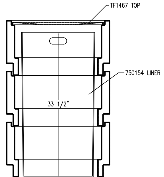
3 SECTION VIEW
