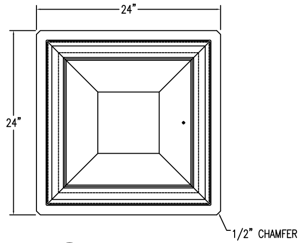
1 TOP VIEW
