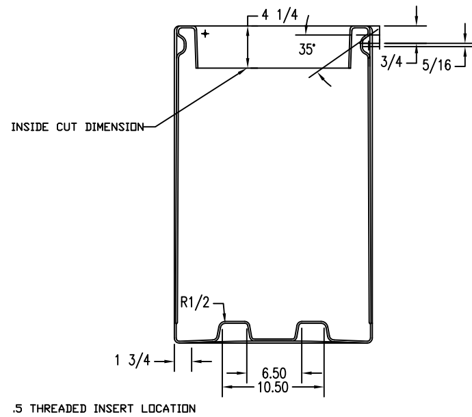
SECTION VIEW CONTAINER
