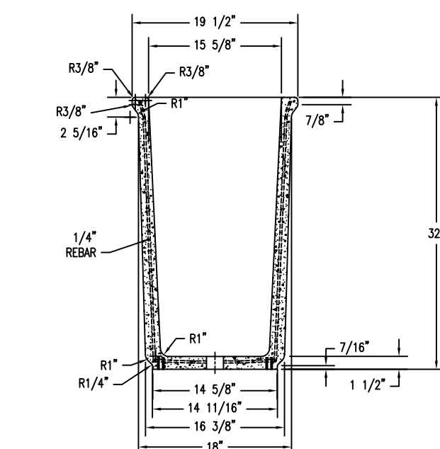
6 SECTION VIEW OF TF1810 WASTE CONTAINER Scale: 1/8" = 1"
