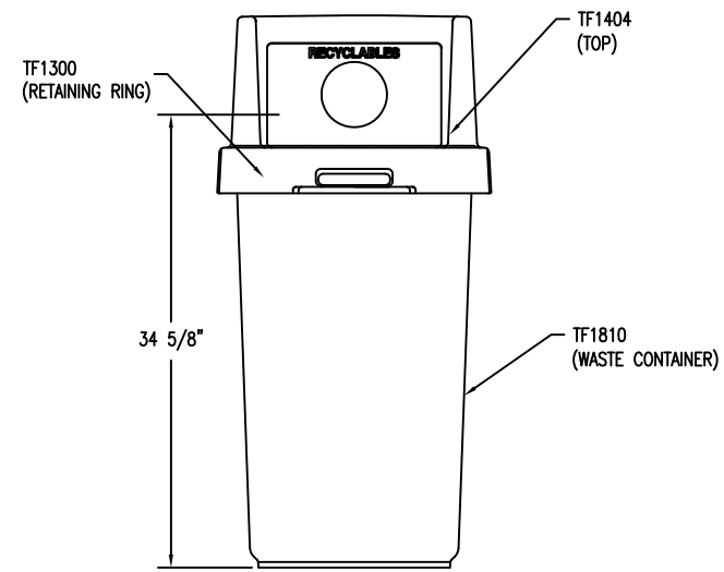
ELEVATION VIEW
