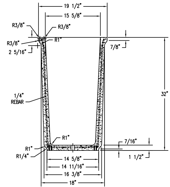
SECTION VIEW
