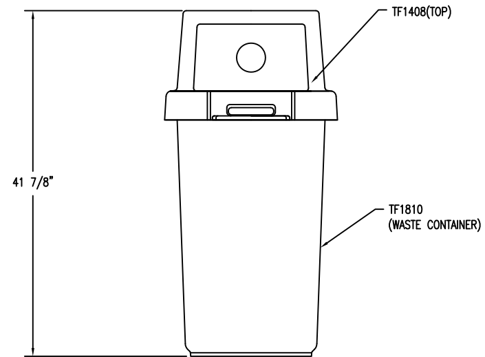
ELEVATION VIEW
