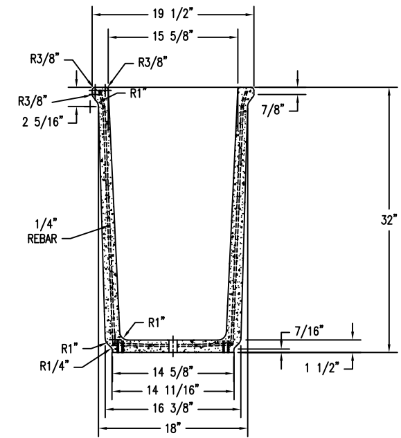
SECTION VIEW
