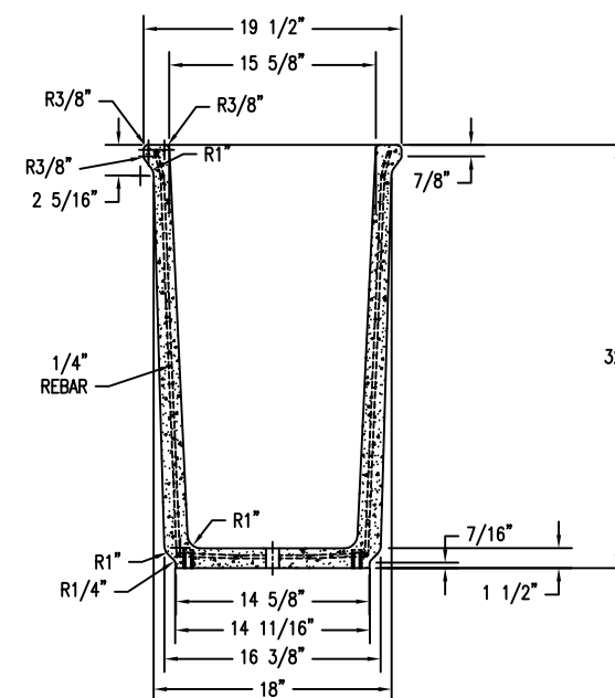
SECTION VIEW
