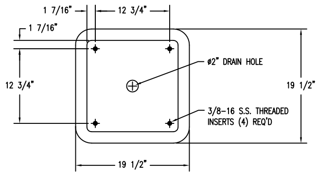
4 BOTTOM VIEW OF TF1810 WASTE CONTAINER Scale: 1/8" = 1"
