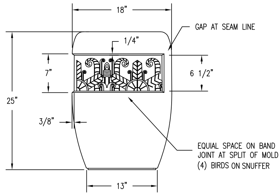
SIDE VIEW
