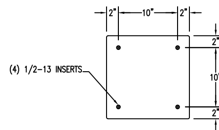
3 BOTTOM VIEW OF SNUFFER
