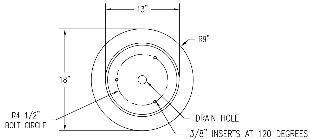
BOTTOM VIEW
