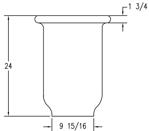
FONT VIEW
