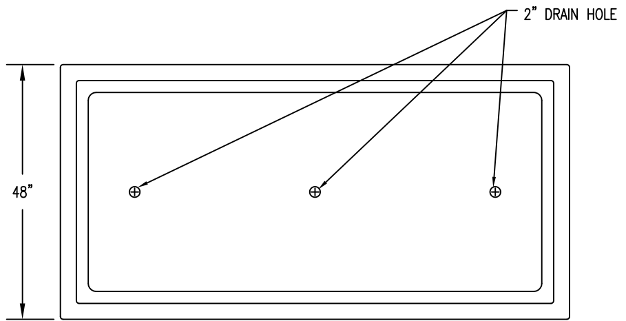
1 TOP VIEW
