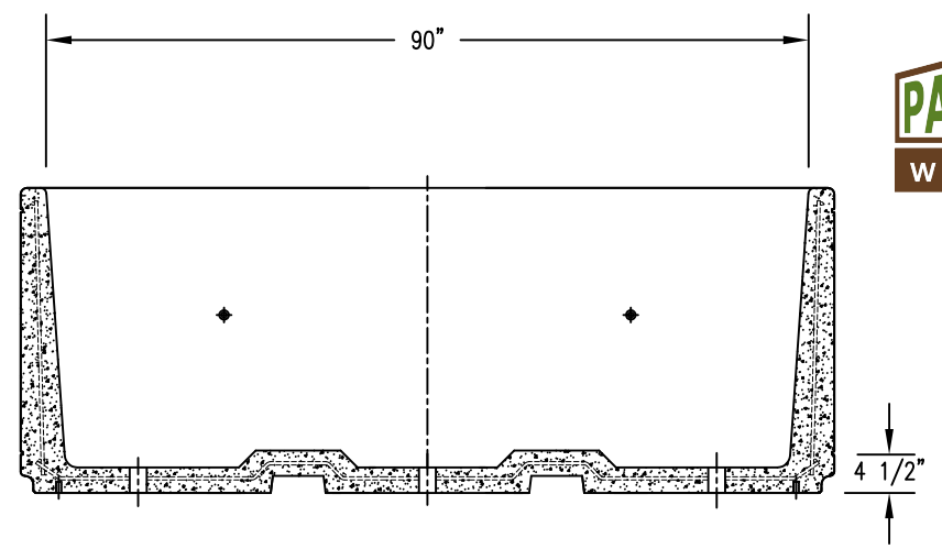
4 CROSS SECTION
