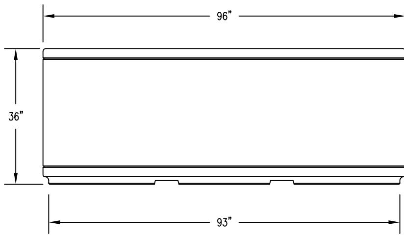
2 ELEVATION VIEW
