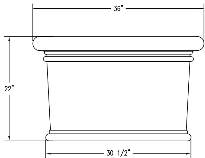
2 ELEVATION VIEW
