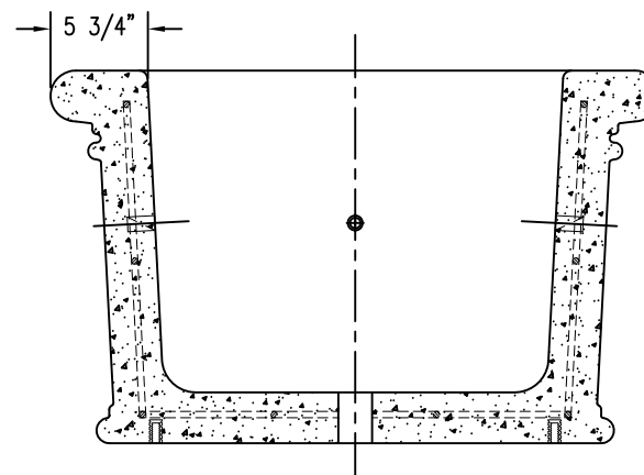
4 CROSS SECTION
