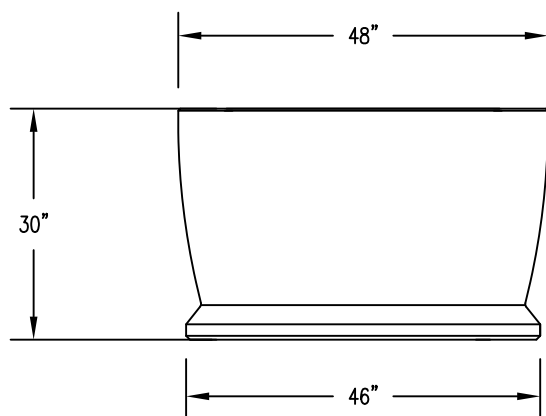
2 ELEVATION VIEW
