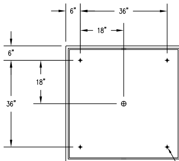
3 BOTTOM VIEW
