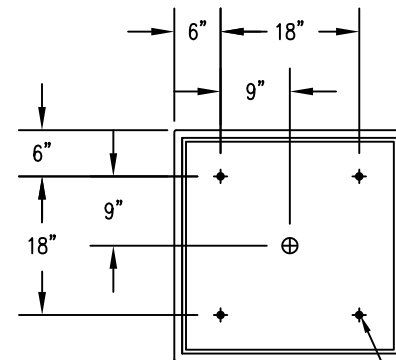
4 CROSS SECTION
