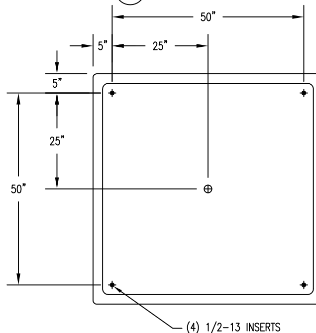
3 BOTTOM VIEW
