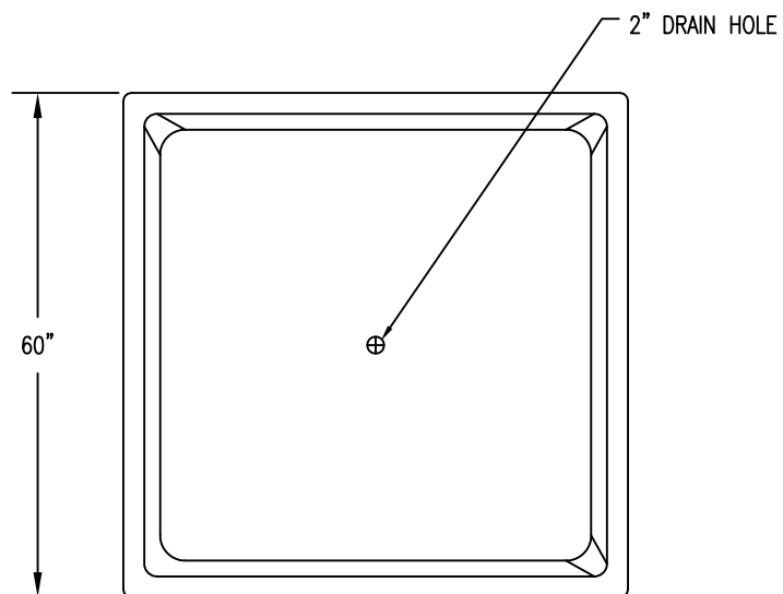
1 TOP VIEW
