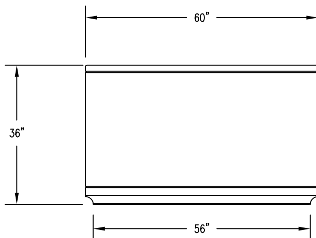
1 TOP VIEW
