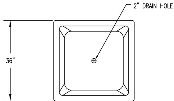
1 TOP VIEW
