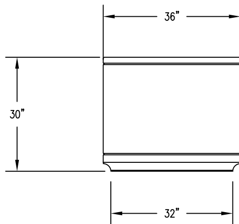
2 ELEVATION VIEW
