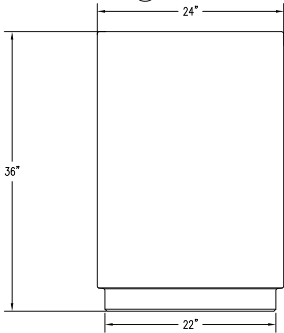
2 ELEVATION VIEW
