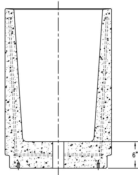
4 CROSS SECTION
