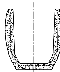
4 CROSS SECTION
