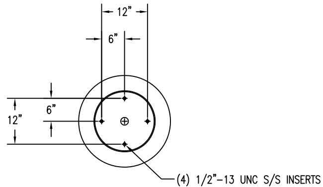
3 BOTTOM VIEW
