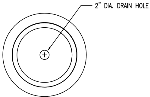
1 TOP VIEW
