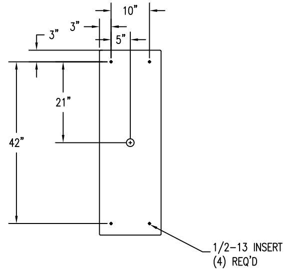
3 BOTTOM VIEW
