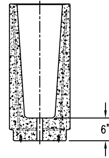
4 CROSS SECTION
