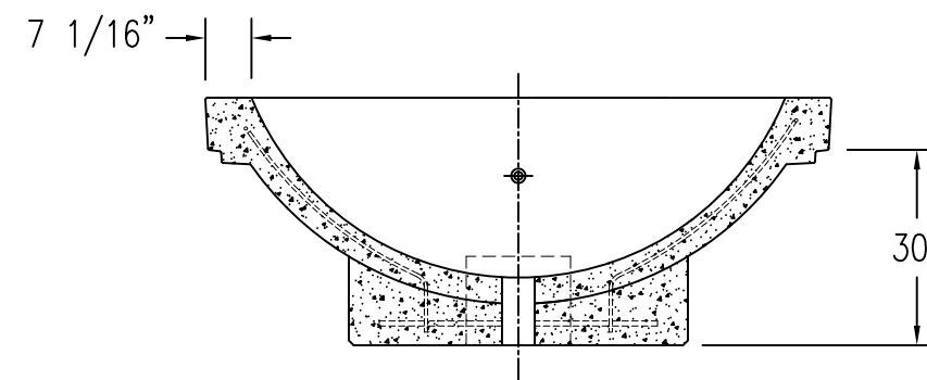
4 CROSS SECTION
