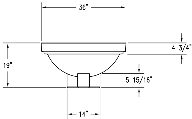
2 ELEVATION VIEW
