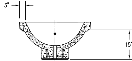
4 CROSS SECTION
