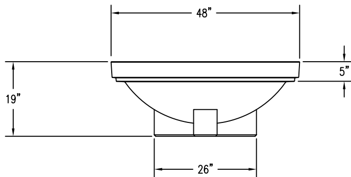
2 ELEVATION VIEW
