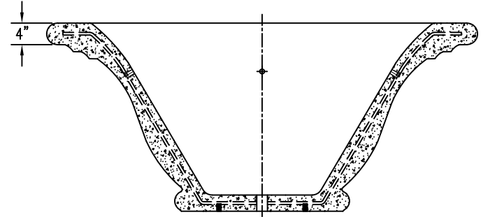
4 CROSS SECTION
