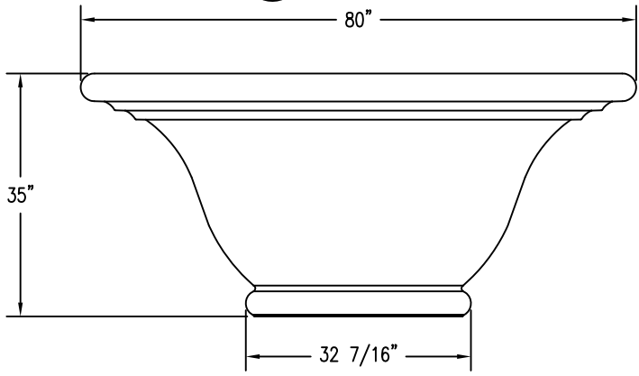
2 ELEVATION VIEW
