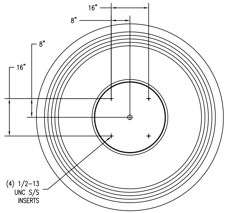
3 BOTTOM VIEW
